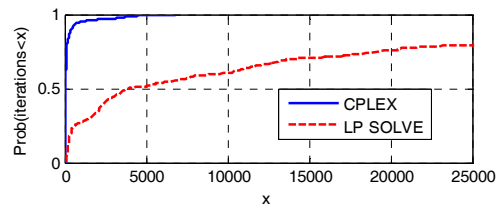
Fig. 6. CDF of the number of iterations executed by the simplex method for 10 users per cell.
