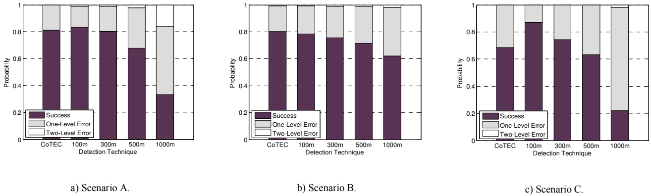
Fig. 8. Congestion level classification success and error rates.
