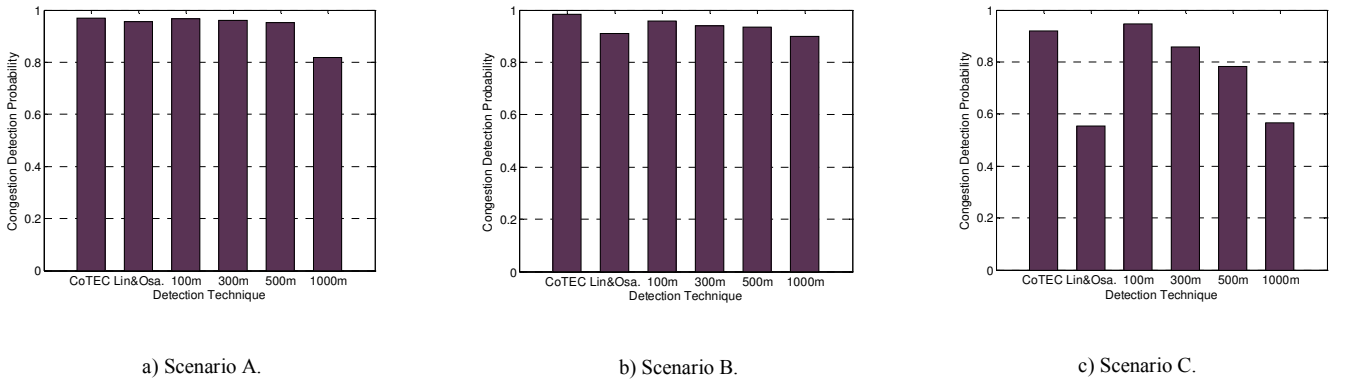
Fig. 6. Congestion detection probability.
