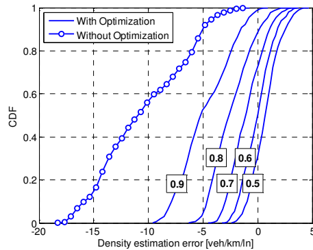
Fig. 3. CDF of the density estimation error.
