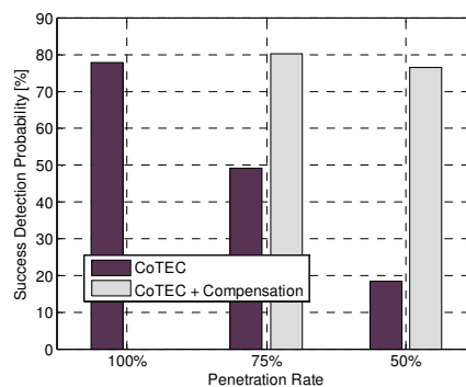
Fig. 10. Success classification rate versus 802.11p/ITS-G5A penetration rate.
