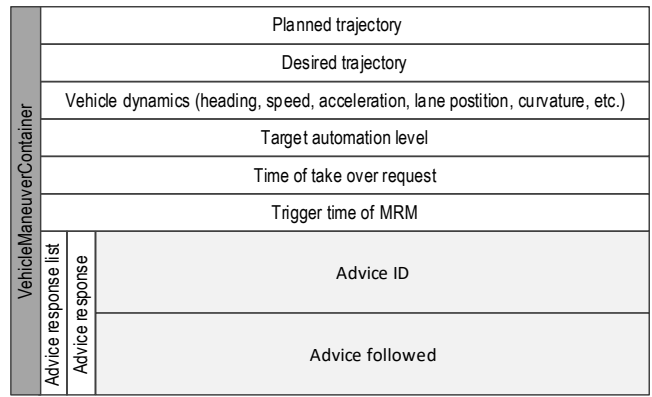
Figure 5. VehicleManeuverContainer .
